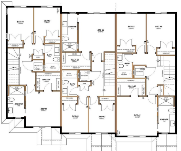
SECOND FLOOR PLAN A: 702 sq ft SECOND FLOOR PLAN A: 721 sq ft SECOND FLOOR PLAN A: 814 sq ft
